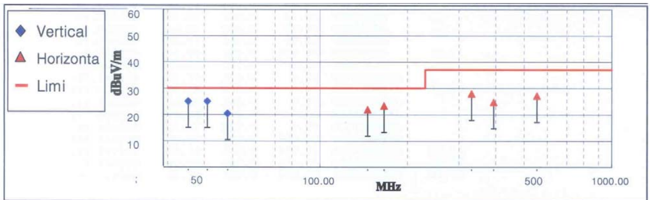
< Fig 5. Radiated emission result _ Digital >
