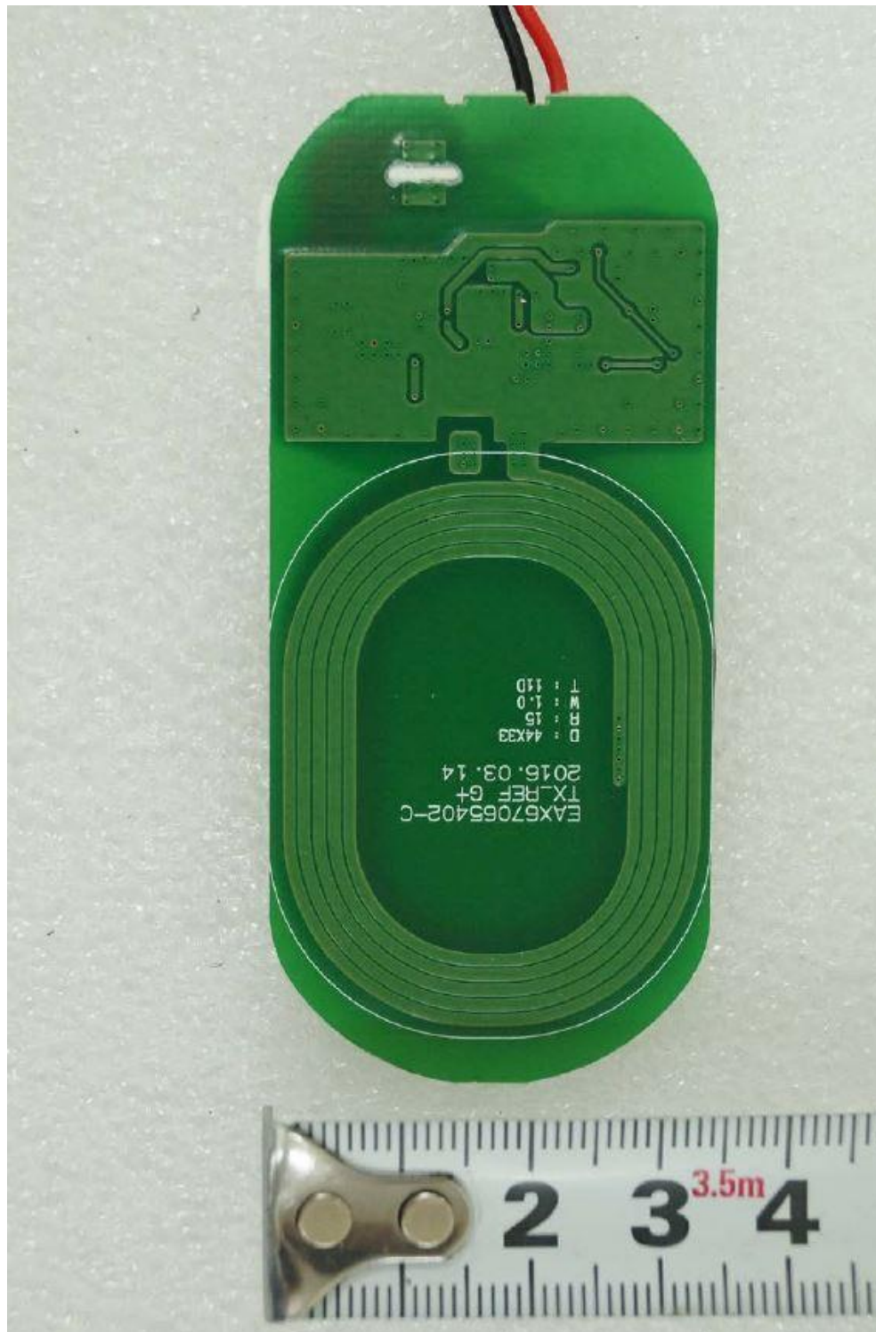
<OLD WPT PCB Section>
