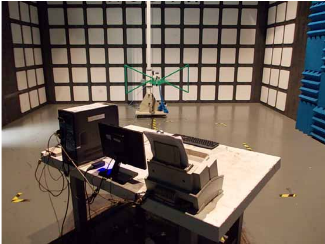
SETUP WITH MAXIMUM DETECTED EMISSION AT HORIZONTAL POLARIZATION (TEST MODE: D-SUB 1366*768@60Hz ADAPTER #1)
