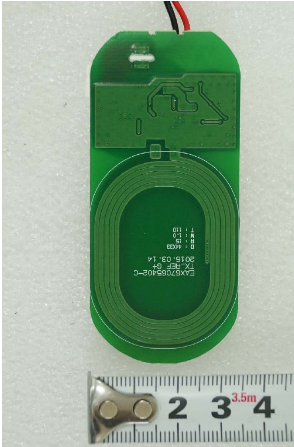
<WPT PCB Section>
