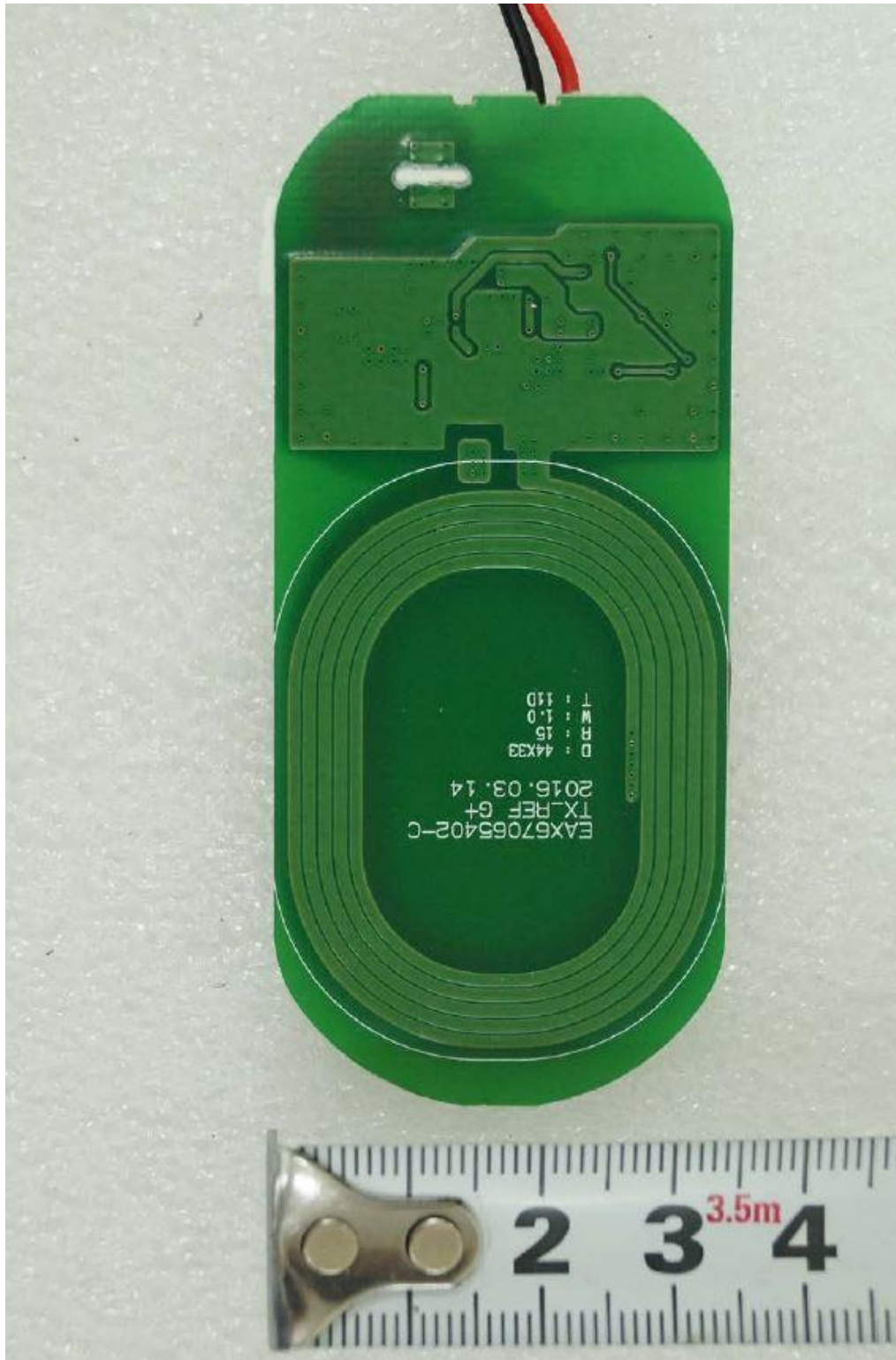
<OLD WPT PCB Section>
