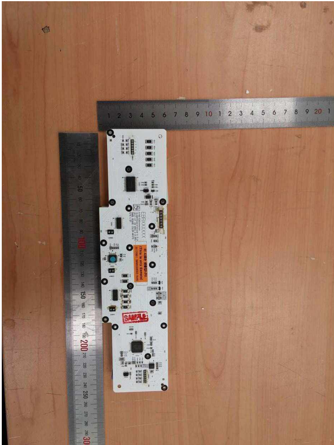
<Display Section-3>
