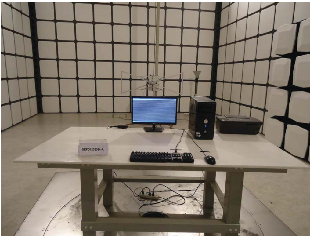
Front View of Radiated Emission Test (30MHz ~ 1000MHz)
