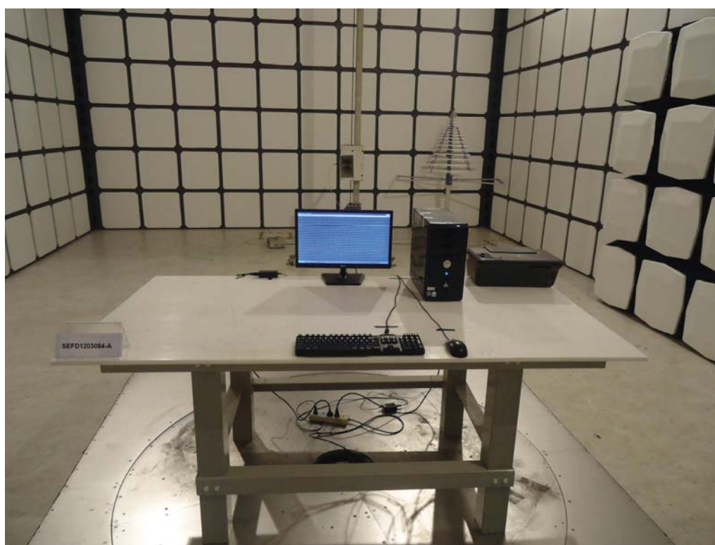
Front View of Radiated Emission Test (1000MHz ~ 18000MHz)
