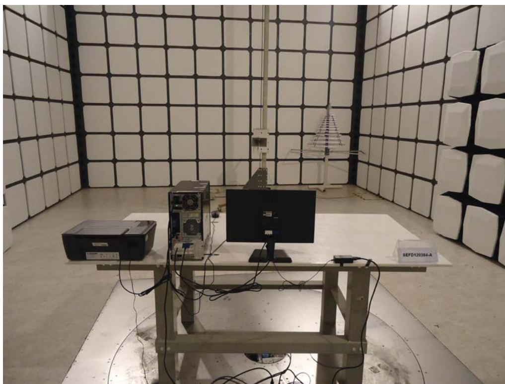
Back View of Radiated Emission Test (1000MHz ~ 18000MHz)
