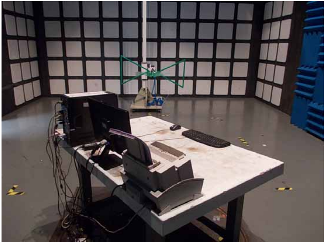
SETUP WITH MAXIMUM DETECTED EMISSION AT HORIZONTAL POLARIZATION (TEST MODE: DVI 1920*1080@60Hz Adapter #1, Panel #1)
