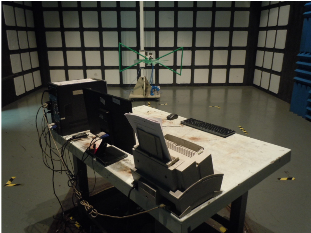
SETUP WITH MAXIMUM DETECTED EMISSION AT HORIZONTAL POLARIZATION (TEST MODE: DVI 1920*1080@60Hz ADAPTER #2, PANEL #2)
