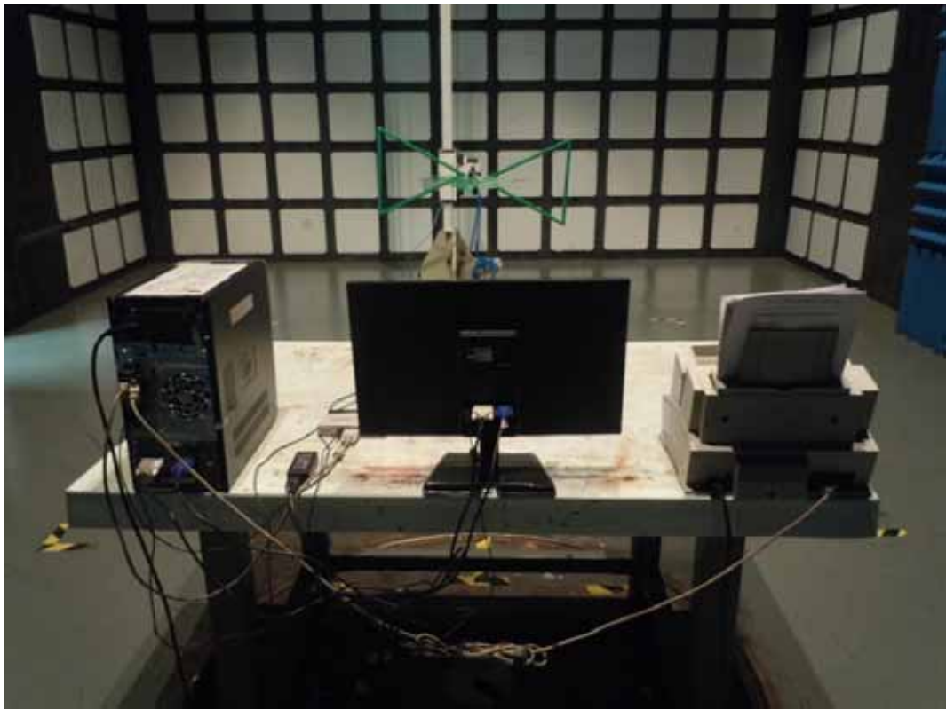
SETUP WITH MAXIMUM DETECTED EMISSION AT HORIZONTAL POLARIZATION (TEST MODE: DVI 1280*1024@75Hz ADAPTER #1)
