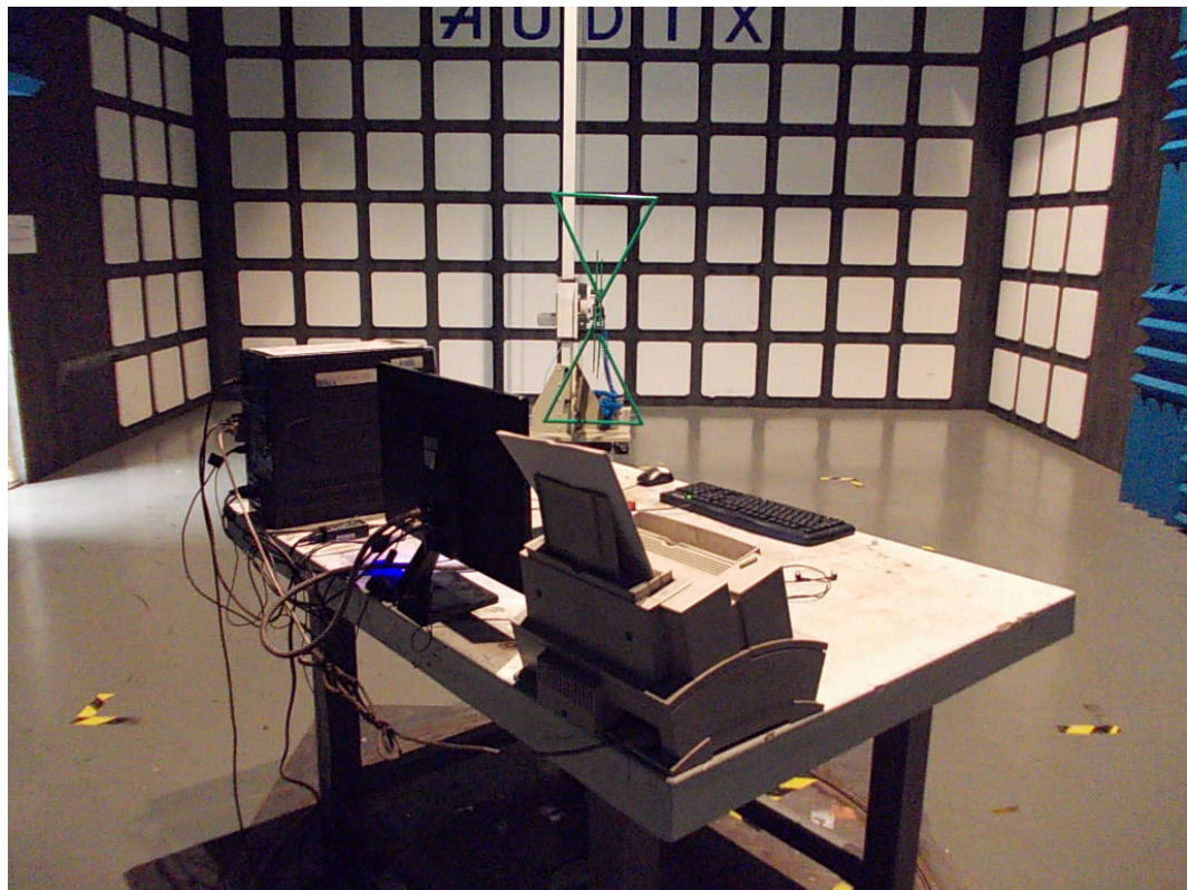
SETUP WITH MAXIMUM DETECTED EMISSION AT VERTICAL POLARIZATION (TEST MODE: DVI 1920*1080@60Hz ADAPTER #1)
