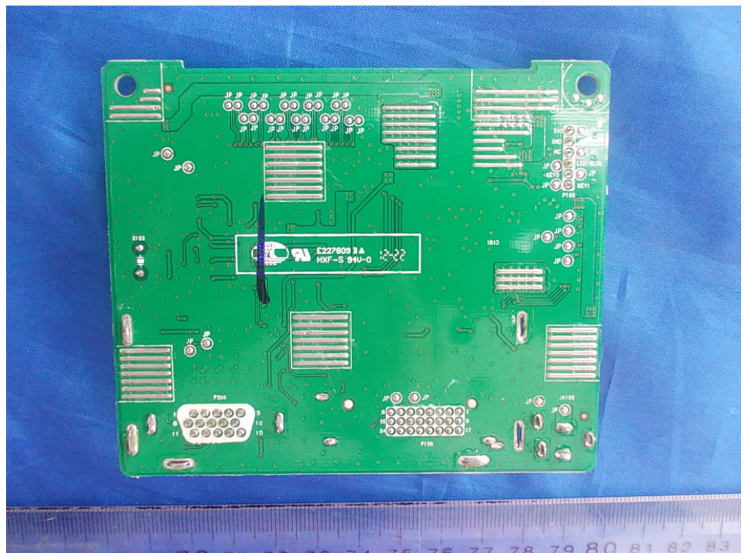
FIGURE 4 LCD MONITOR (M/N: E2442TA) MAIN BOARD (SOLDERED SIDE)
