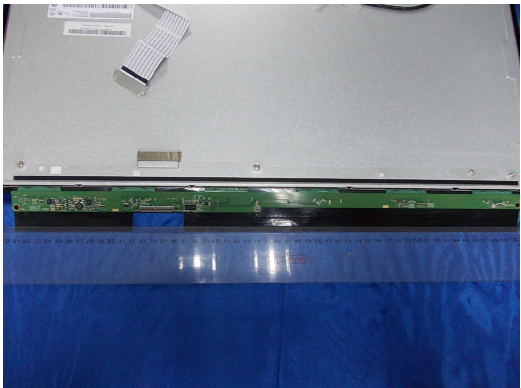
FIGURE 9 LCD MONITOR (M/N: E2442TA) LCD PANEL BOARD (SOLDERED SIDE)
