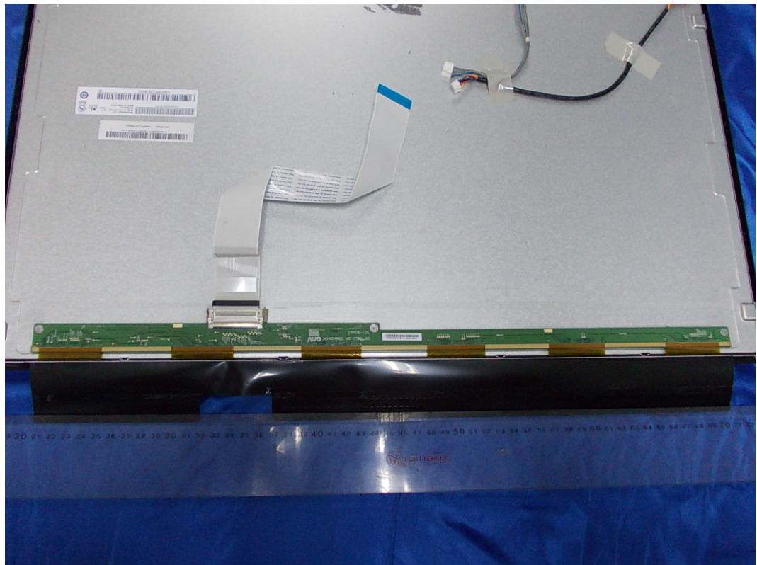
FIGURE 8 LCD MONITOR (M/N: E2442TA) LCD PANEL BOARD (COMPONENT SIDE)
