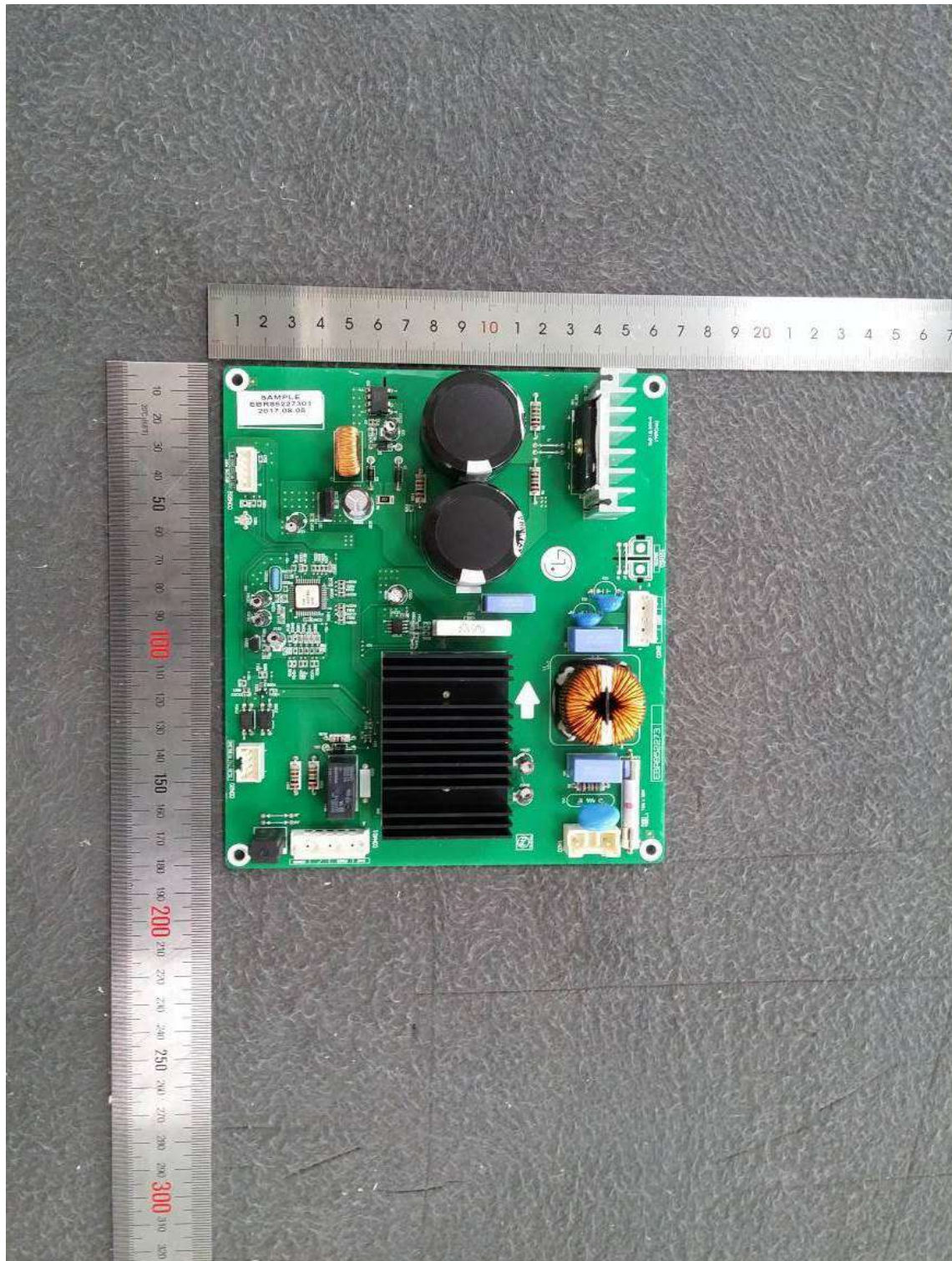
OLD Item_<Sub PCB Section-2>
