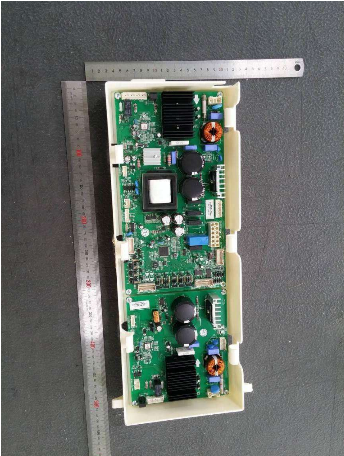
OLD Item_<Main PCB Section-1>
