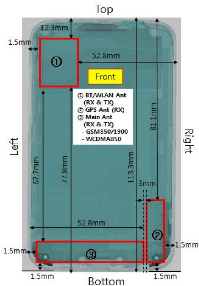
Figure 13.1 Identification of Sides for SAR Testing
