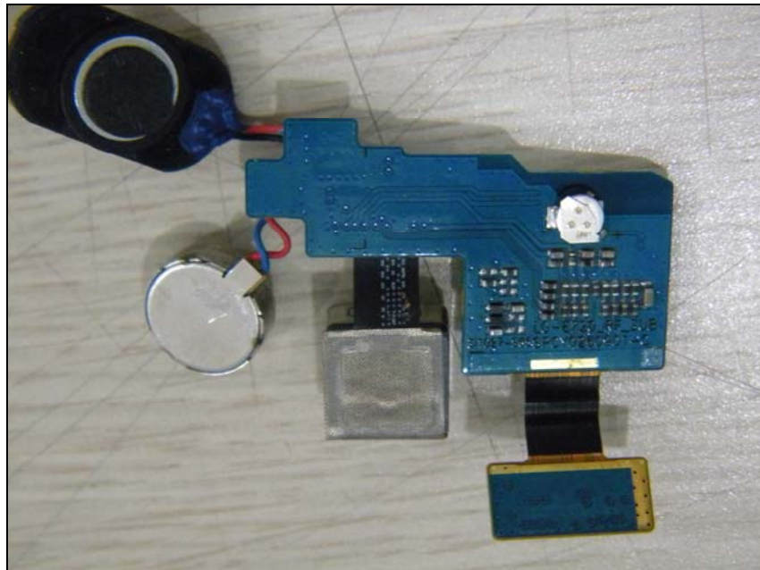
Bottom view of RF Sub board
