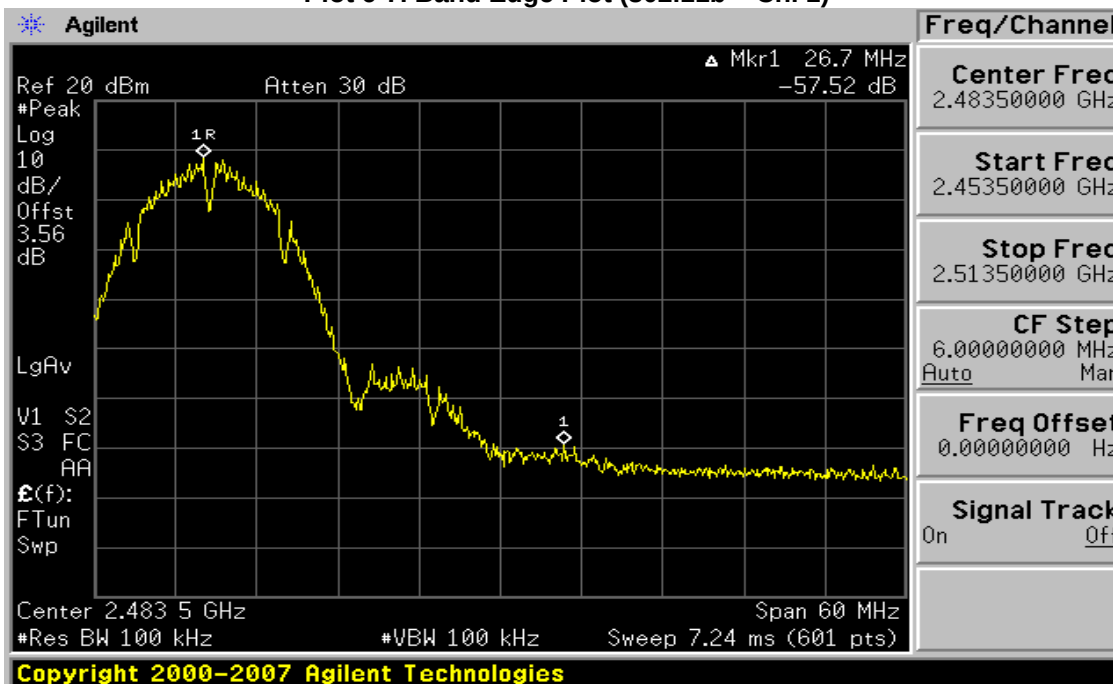
Plot 6-8. Band Edge Plot (802.11b – Ch. 11)
