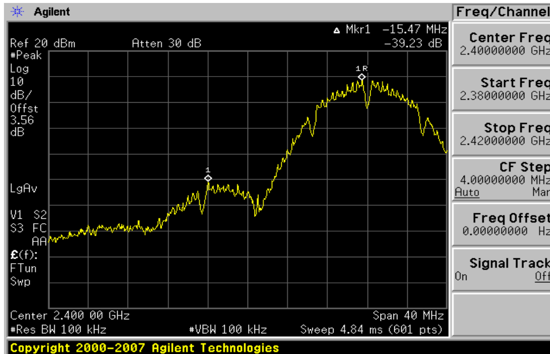
Plot 6-7. Band Edge Plot (802.11b – Ch. 1)
