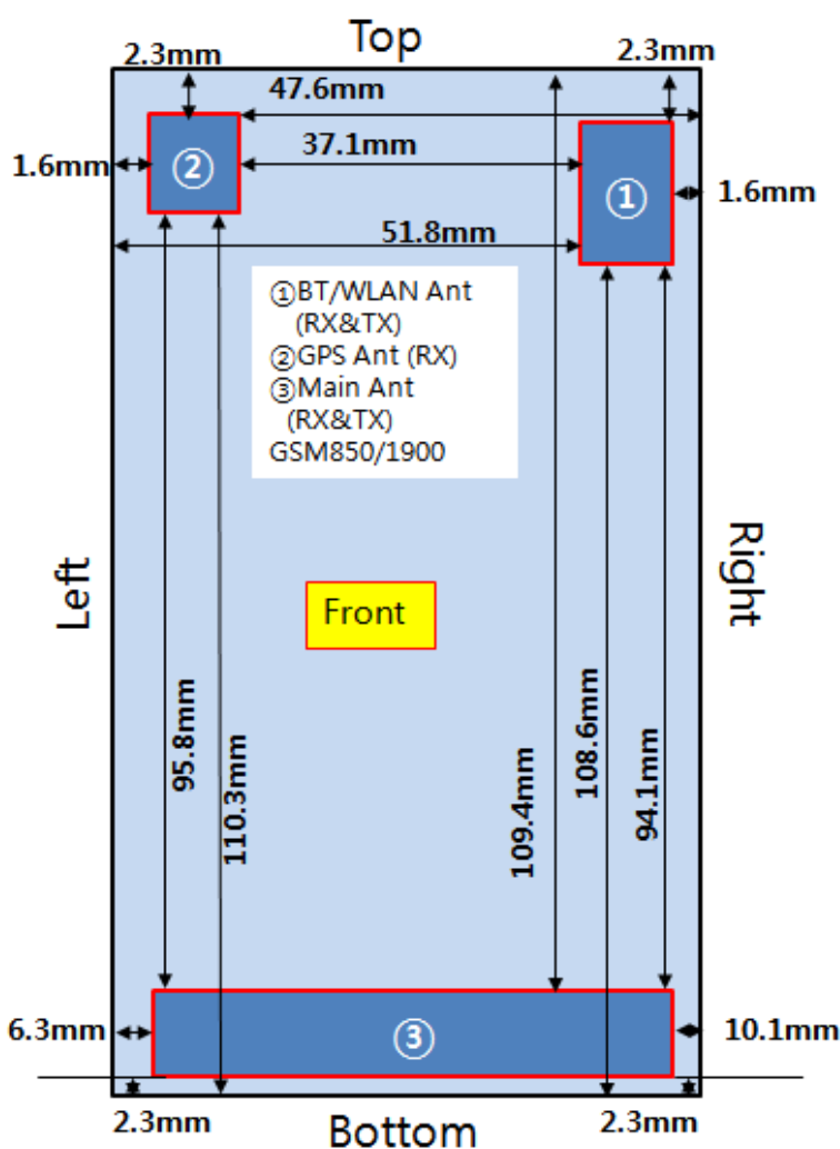
Figure 12.1 Identification of Sides for SAR Testing
