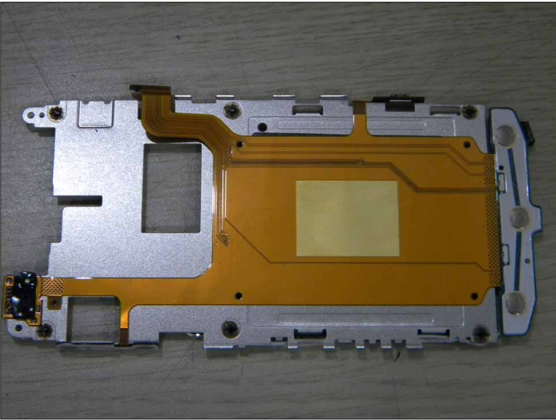
RF Key board Front
