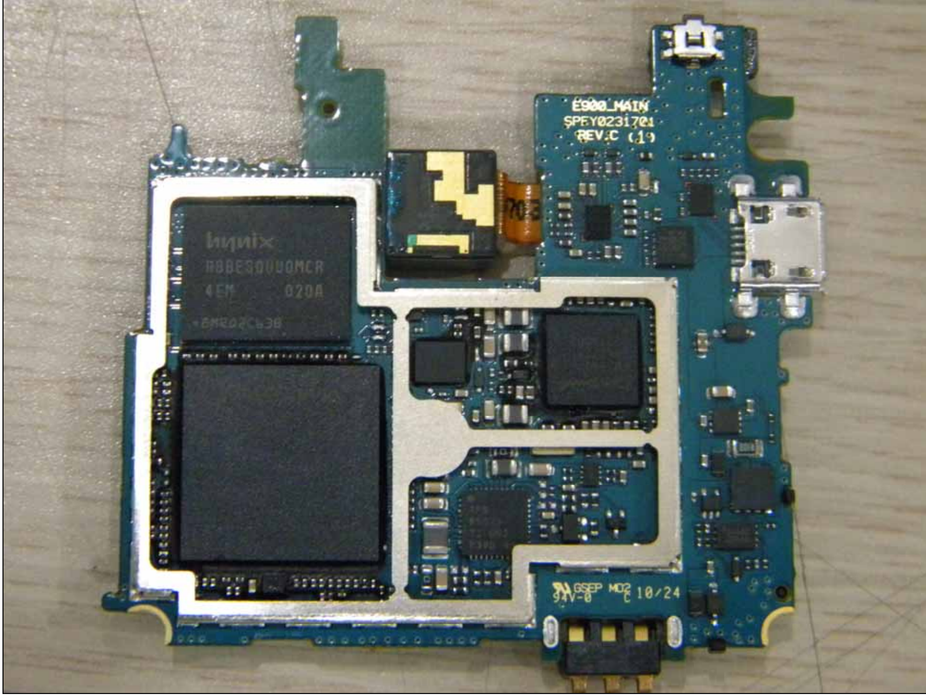
Main board Rear
