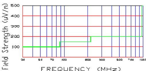
Figure 6-1. 3-Meter Limits
