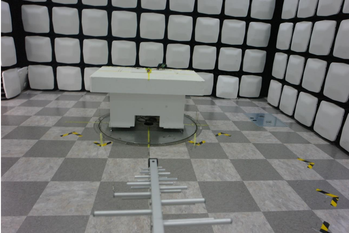
RFID Radiated Test Setup Photo for 30 MHz ~ 1 GHz:
