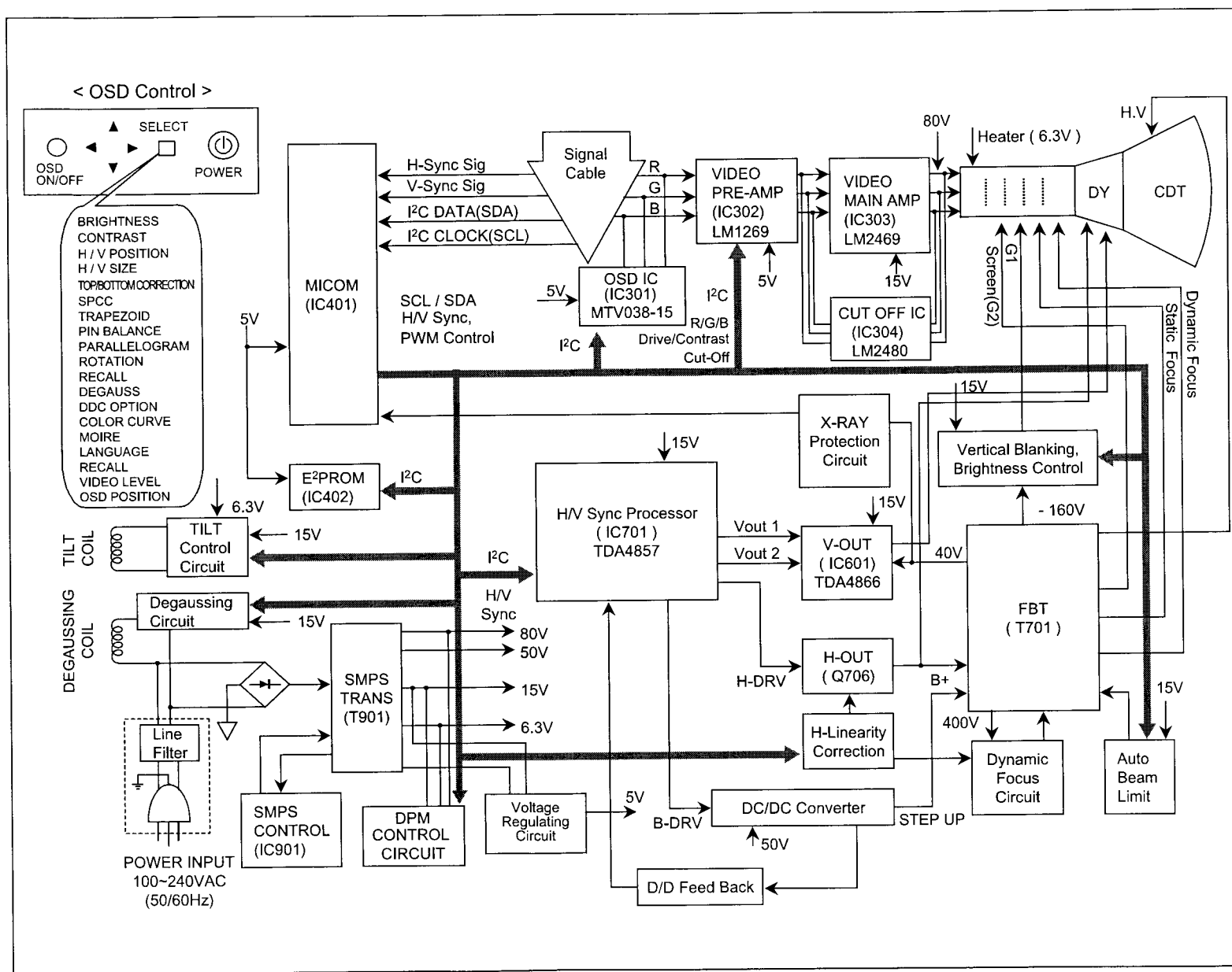
BLOCK DIAGRAM
