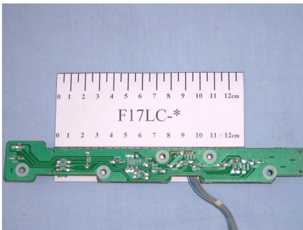
FIGURE 9 COLOR MONITOR (M/N:F17LC-*) CONTROL PANEL BOARD (SOLDERED SIDE)
