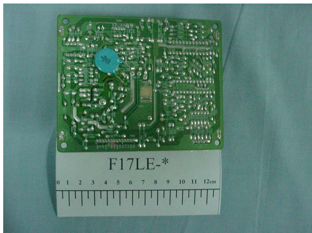
FIGURE 8 COLOR MONITOR (M/N: F17LE-*) CRT BOARD (SOLDERED SIDE)
