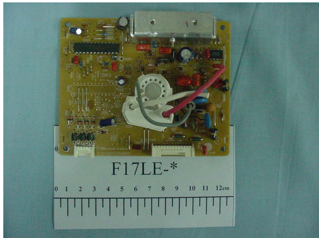
FIGURE 7 COLOR MONITOR (M/N: F17LE-*) CRT BOARD (COMPONENT SIDE)
