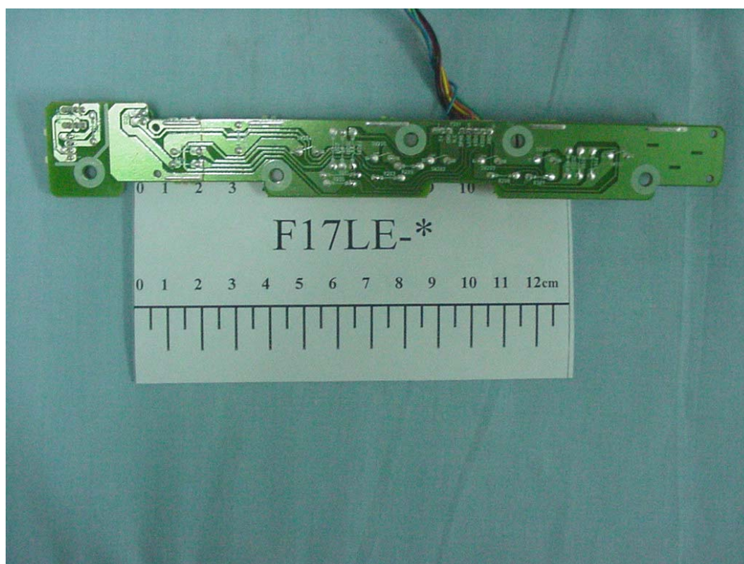
FIGURE 10 COLOR MONITOR (M/N: F17LE-*) CONTROL PANEL BOARD (SOLDERED SIDE)
