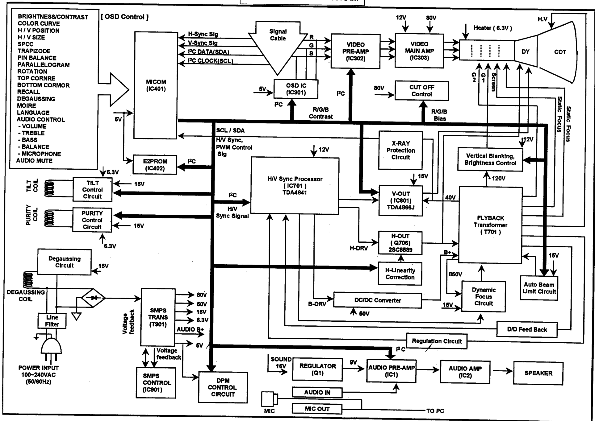
FM776F * BLOCK DIAGRAM
