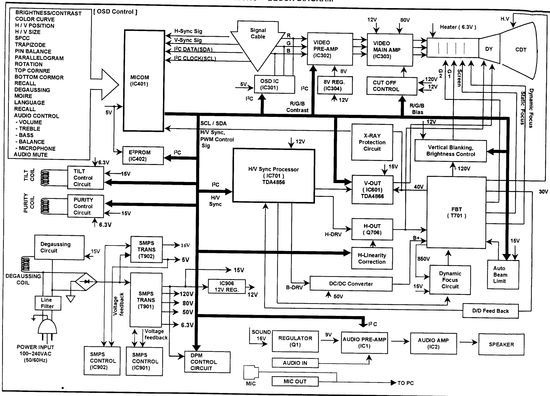
FM77NC * BLOCK DIAGRAM
