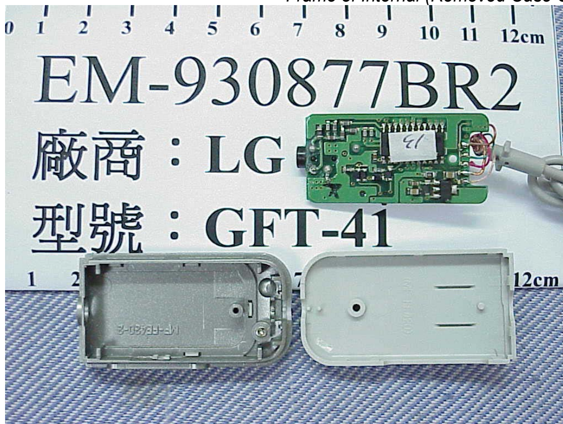
Figure 3 Frame of Internal (Removed Case Covers)
