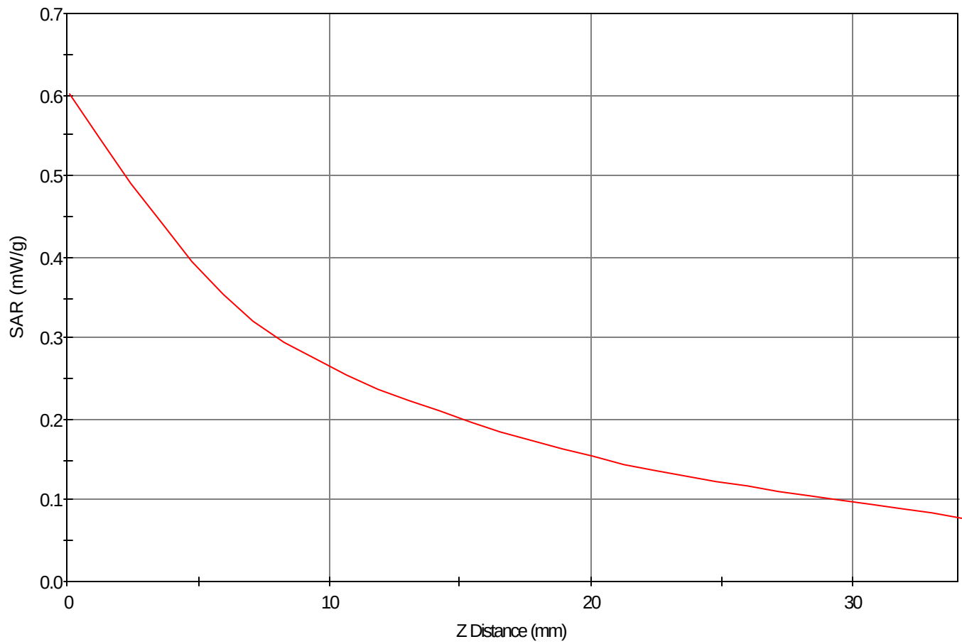
SAR - Z Axis at Hotspot x:0.0 y:15.0
