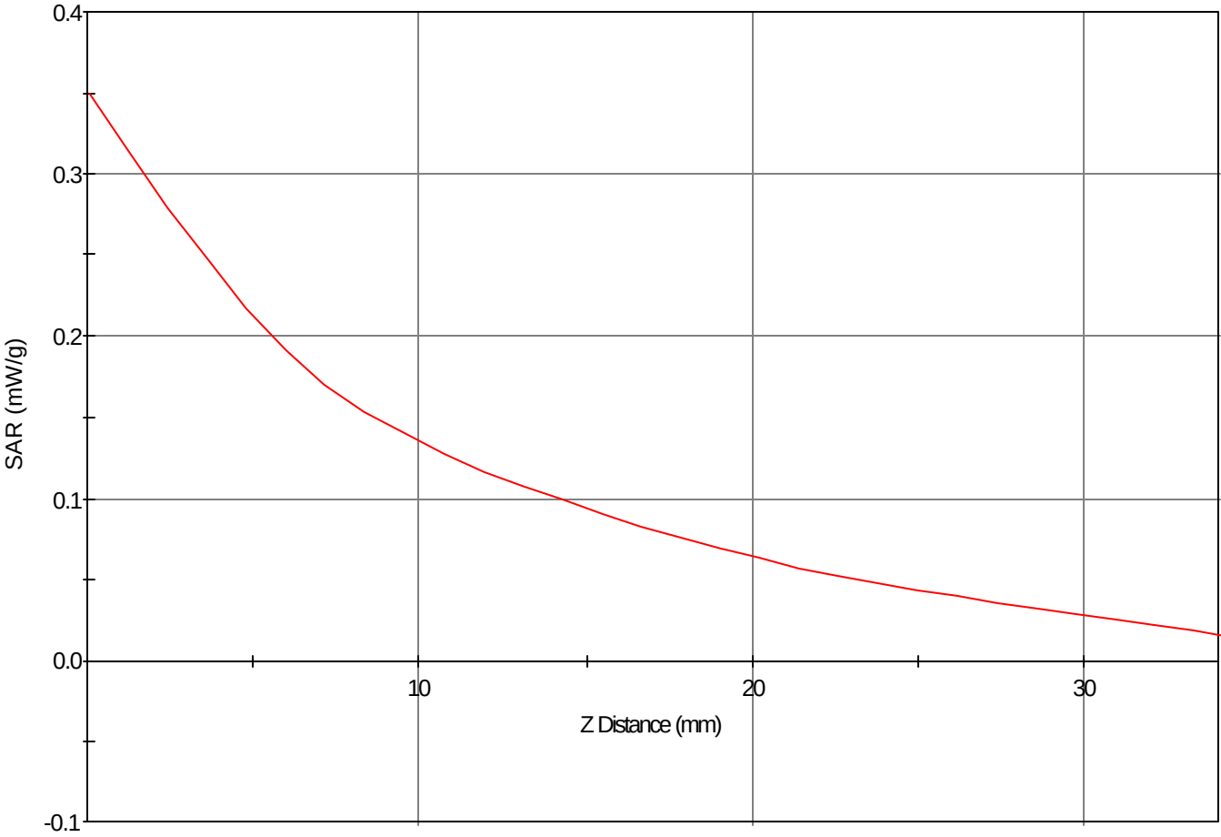
SAR - Z Axis at Hotspot x:3.0 y:9.0
