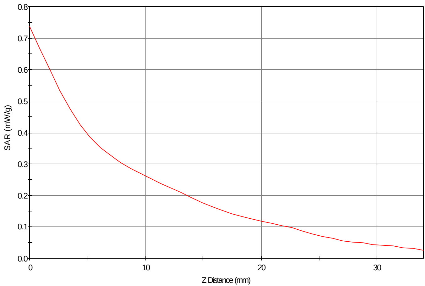
SAR - Z Axis at Hotspot x:-4.0 y:13.0
