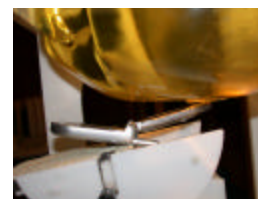
Figure A.8 Left Head SAR Test Setup -- Ear / 15° Tilt Position --
