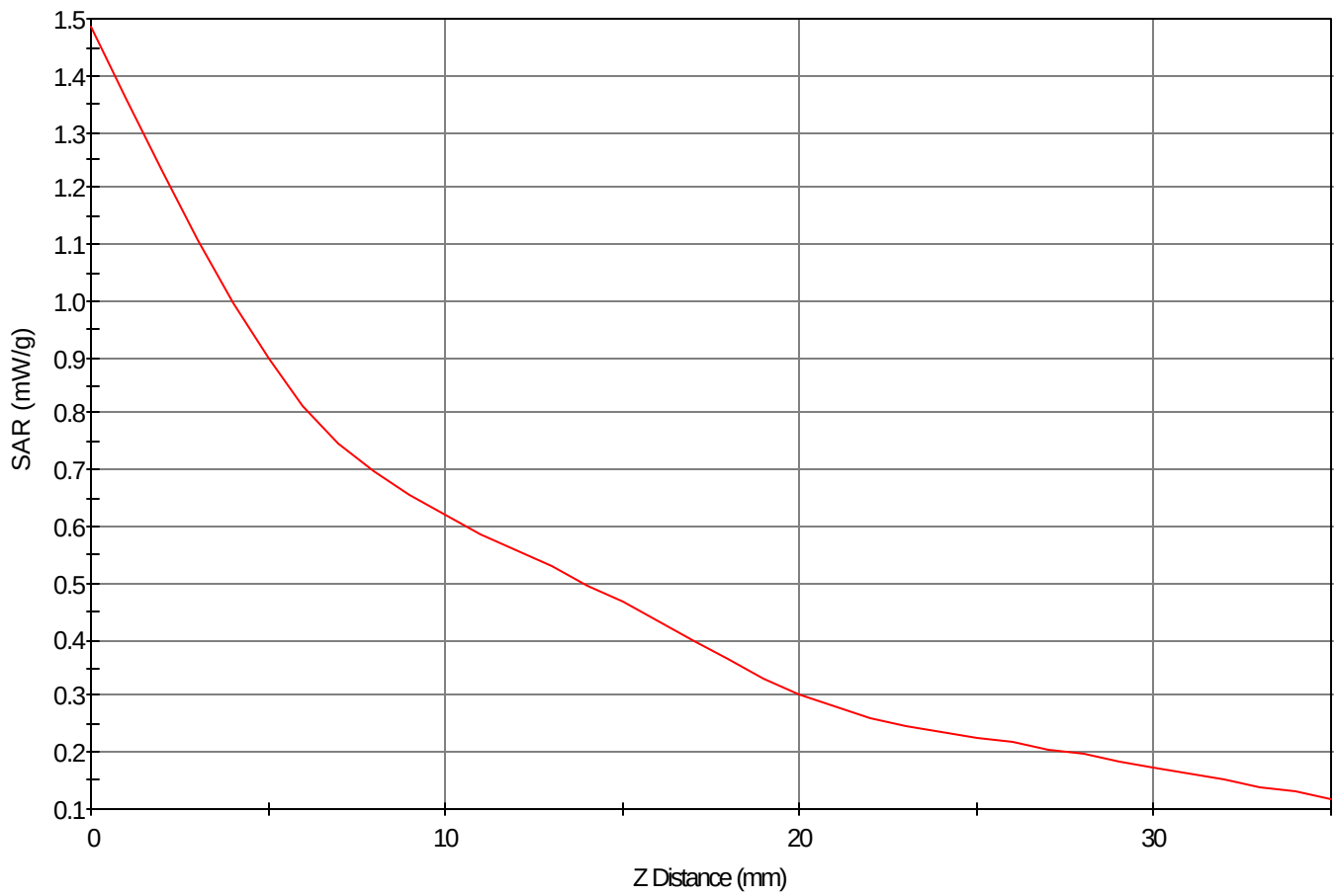
SAR - Z Axis at Hotspot x:75.0 y:1.0
