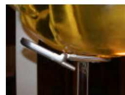
Figure A.7 Left Head SAR Test Setup -- Cheek / Touch Position --
