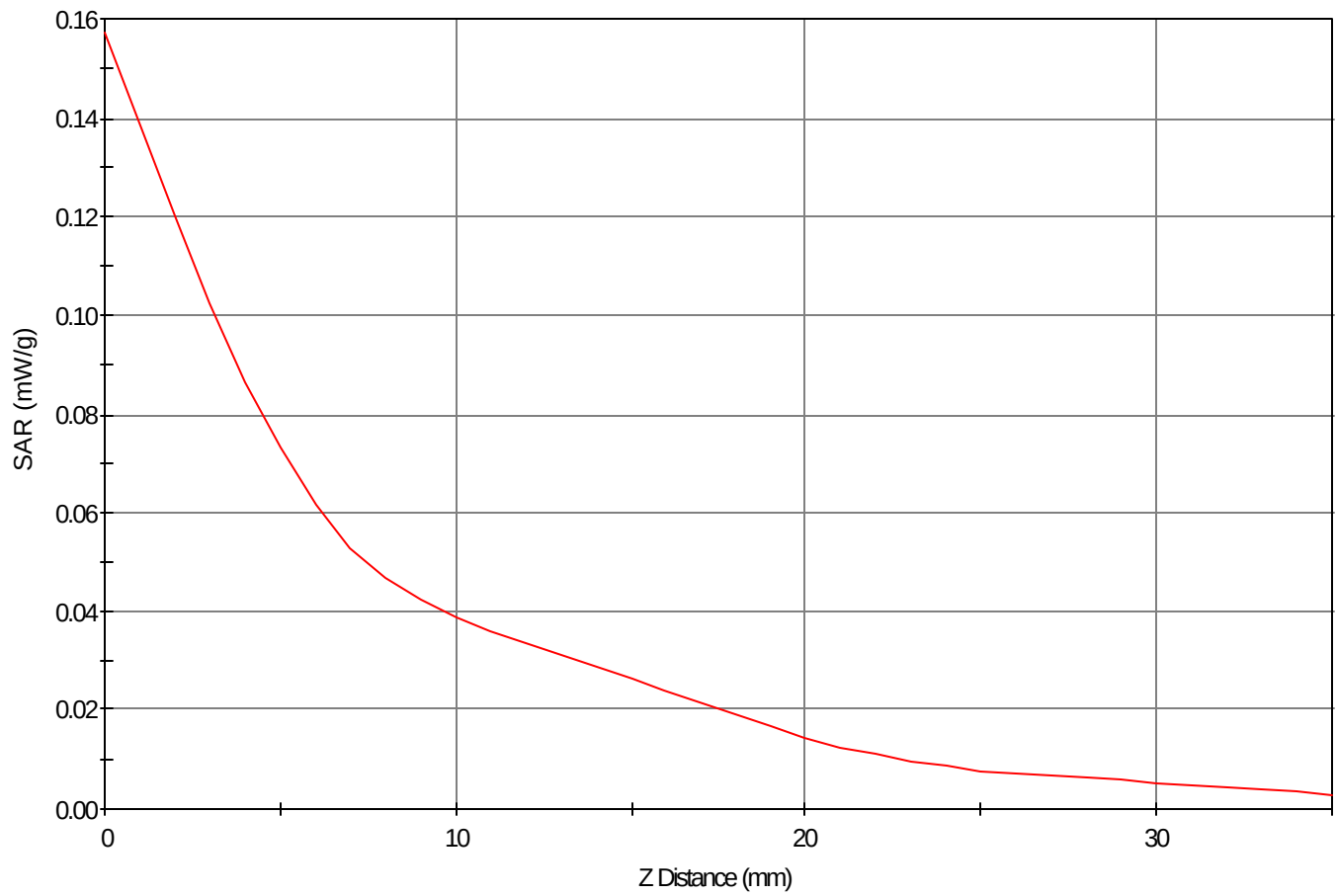
SAR - Z Axis at Hotspot x:17.0 y:12.0
