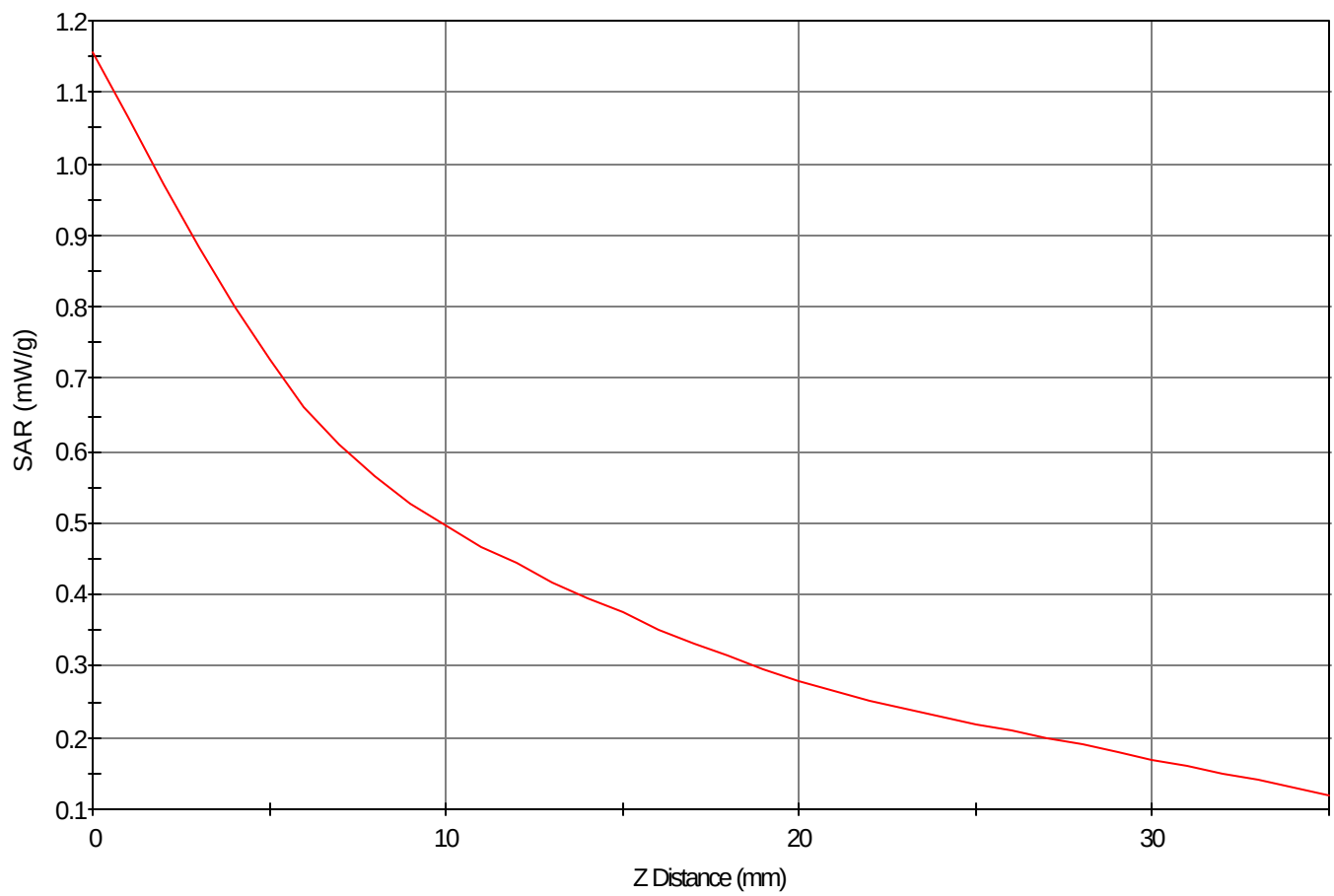
SAR - Z Axis at Hotspot x:72.0 y:10.0
