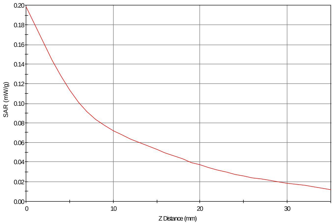
SAR - Z Axis at Hotspot x:84.0 y:10.0
