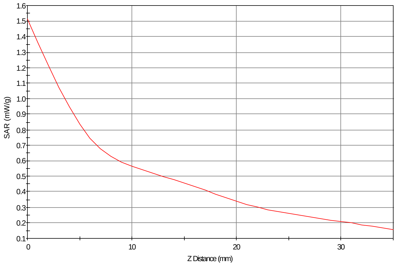
SAR - Z Axis at Hotspot x:65.0 y:9.0
