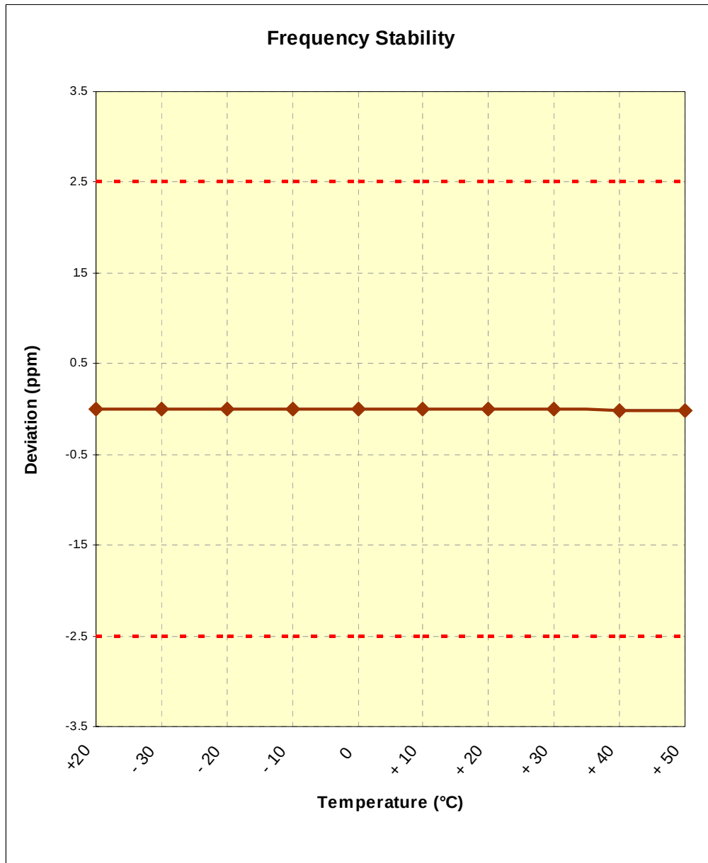
Figure 6-1. Frequency Stability Graph (AWS WCDMA Mode – Ch. 1412)
