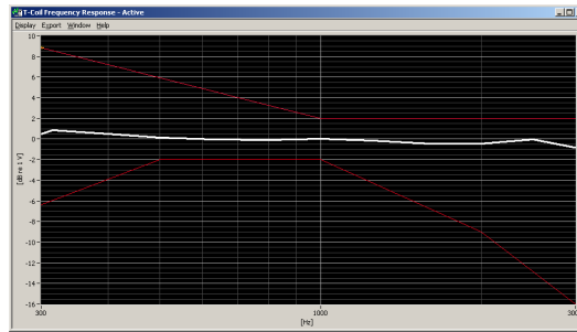
Figure 7-1 Axial Frequency Response
