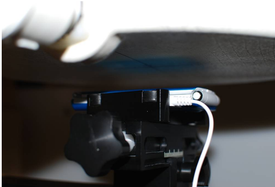
Figure 19-7 SAR Test Setup Photo 7
