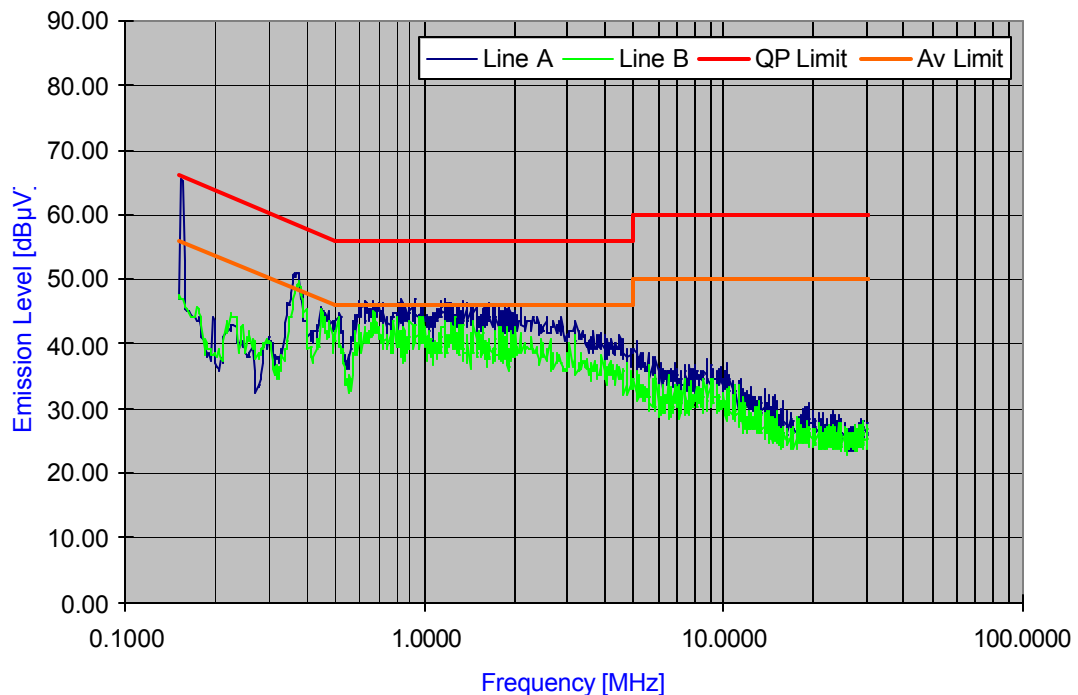
Plot 6-24. Line Conducted Plot with 802.11g
