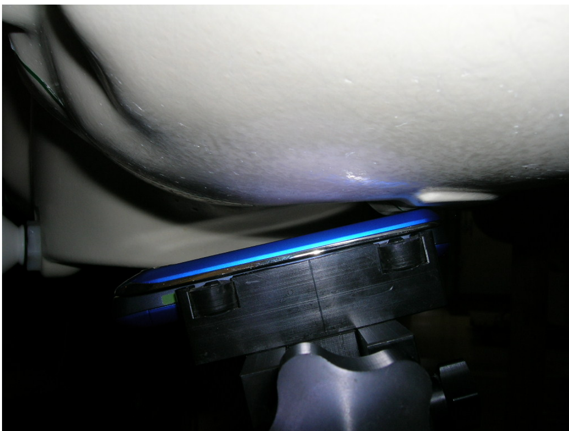
Figure 6 Left Tilt
