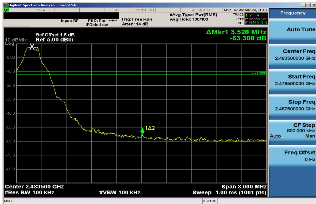
Plot 6-5. Band Edge Plot (Bluetooth – Ch. 78)
