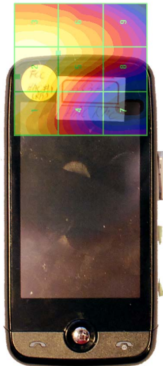
Figure 16-4 E-Field WD Scan overlay
