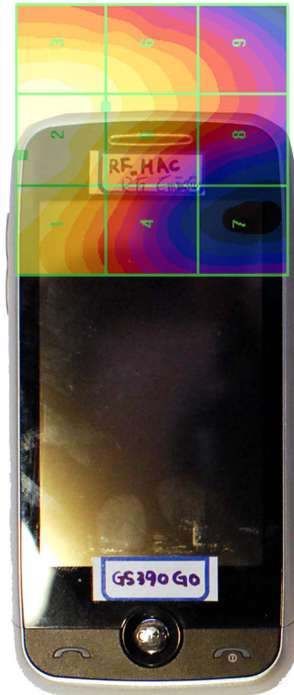
Figure 16-4 E-Field WD Scan overlay
