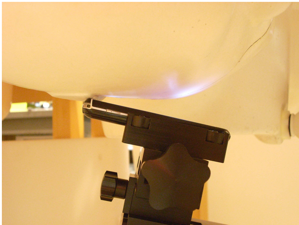
Figure 19-2 SAR Test Setup Photo 2
