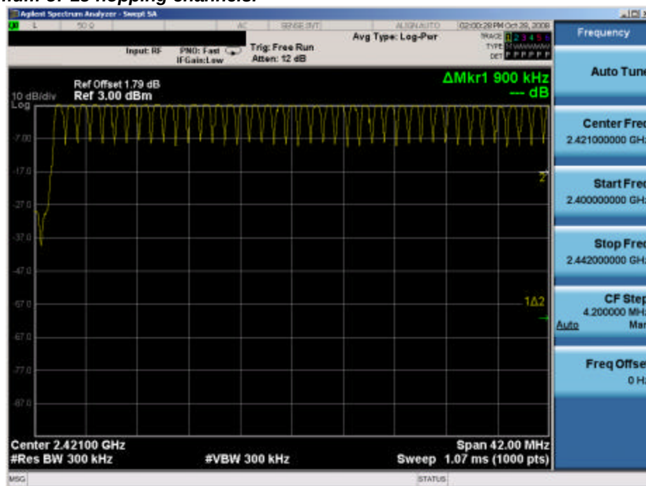
Plot 6-10. Low End Spectrum Channel Hopping Plot (Bluetooth)
