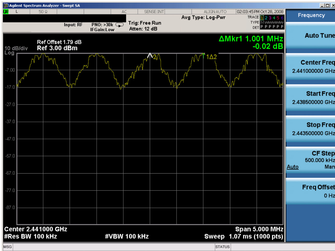
Plot 6-8. Channel Spacing Plot (Bluetooth)
