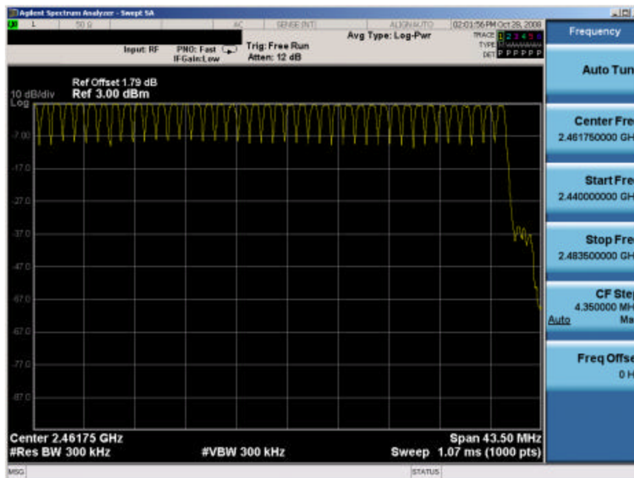
Plot 6-11. High End Spectrum Channel Hopping Plot (Bluetooth)
