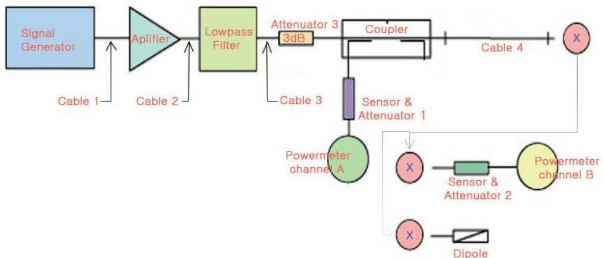
Figure 2.1 Dipole Validation Test Setup
