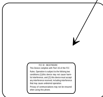
EUT Base Bottom View
