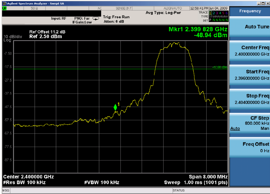
Plot 6-6. Band Edge Plot (Bluetooth 2.0 with Enhanced Data Rate – Ch. 0)
