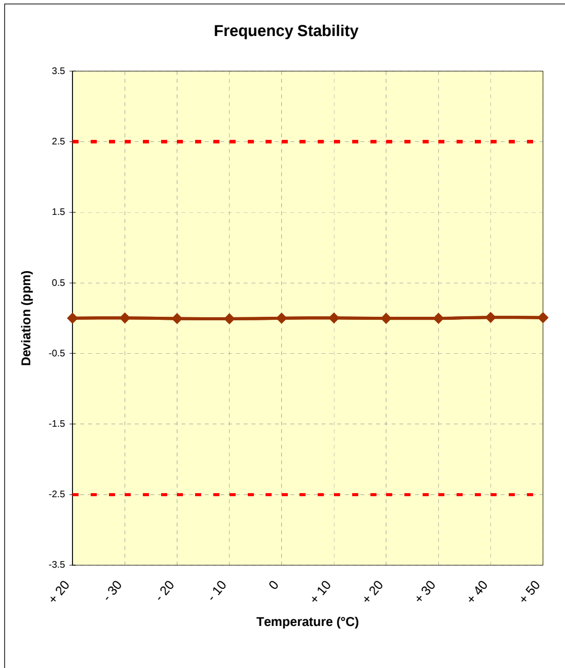
Plot 6-3. Frequency Stability Graph (PCS GSM Mode – Ch. 661)
