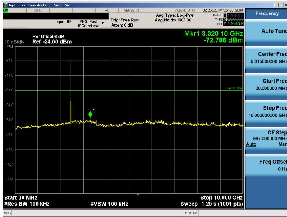
Plot 6-14. Conducted Spurious Plot (Bluetooth – Ch. 39)
