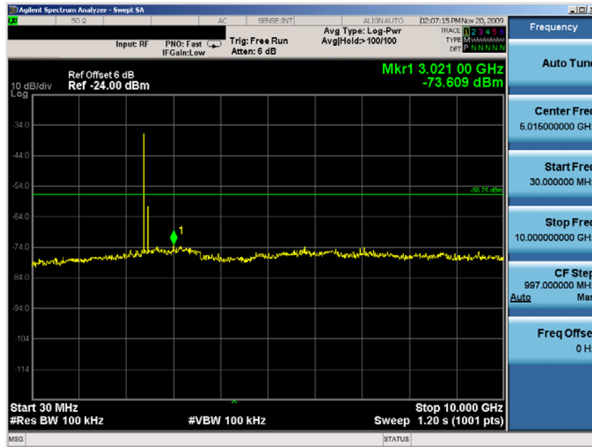
Plot 6-12. Conducted Spurious Plot (Bluetooth – Ch. 0)
