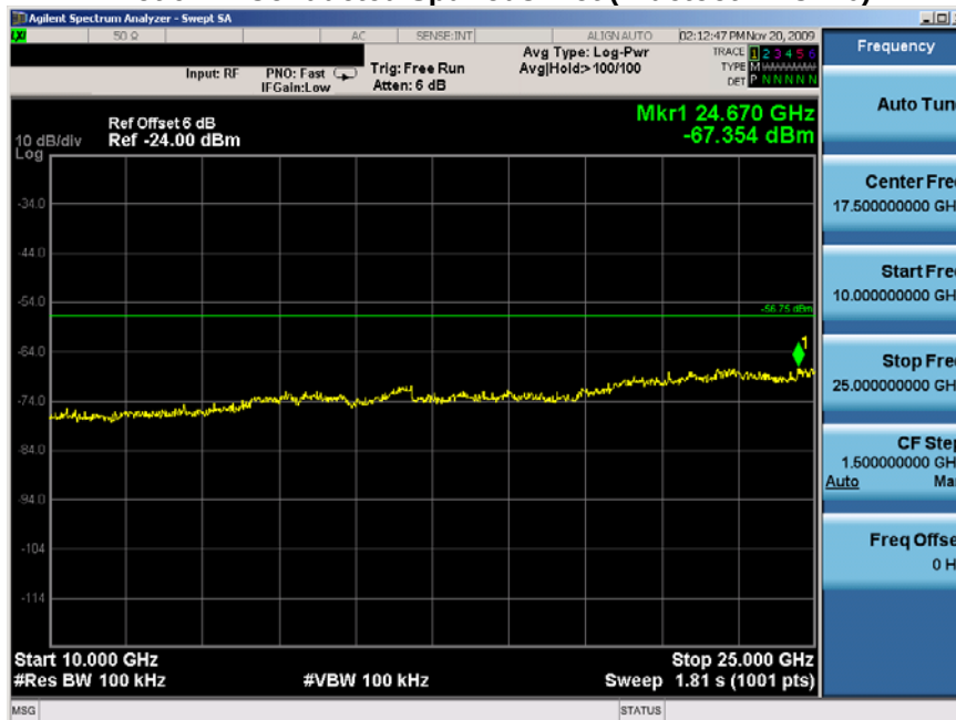
Plot 6-13. Conducted Spurious Plot (Bluetooth – Ch. 0)
