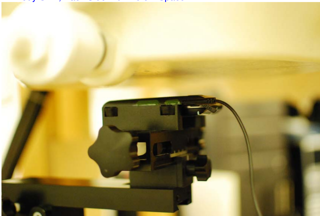
12.Body SAR, Back Side with 2.0 cm Space
