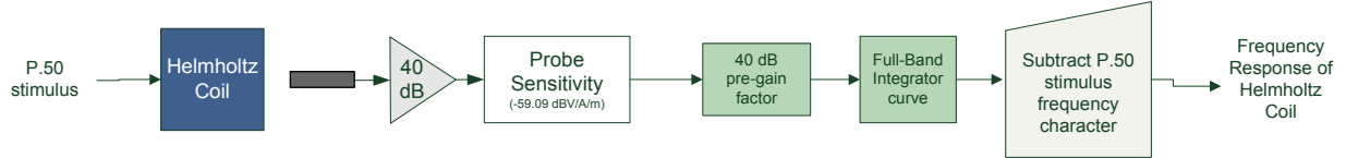
Figure 5-7 Frequency Response Validation
