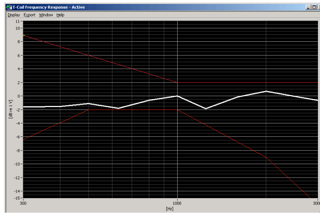
Figure 7-1 Axial Frequency Response
