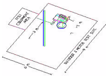
Figure 3-3. Turntable and System Setup
