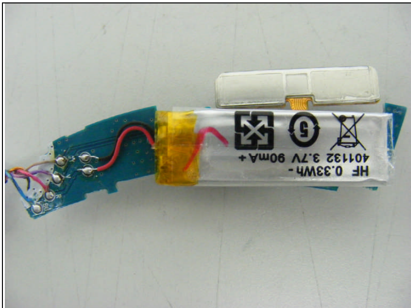
Bottom view of Sub PCB (with battery)
