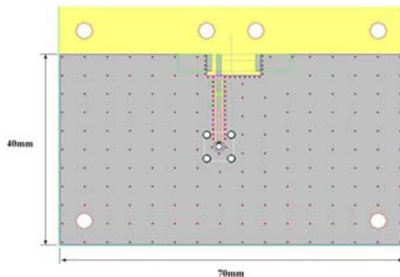
Test Fixture Loss 0.2~0.3 dB
