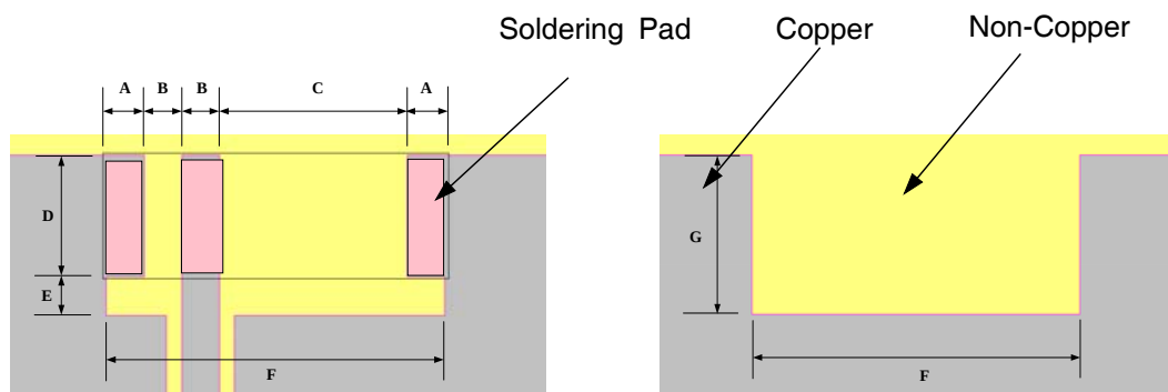
Top Pattern
