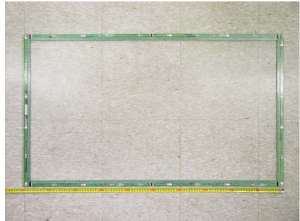
(Rear) Touch screen board
