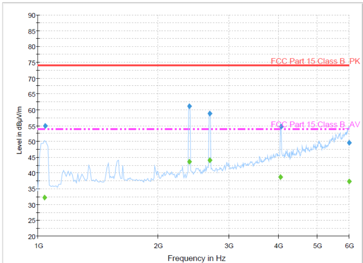
Radiated emission_above 1GHz_T
